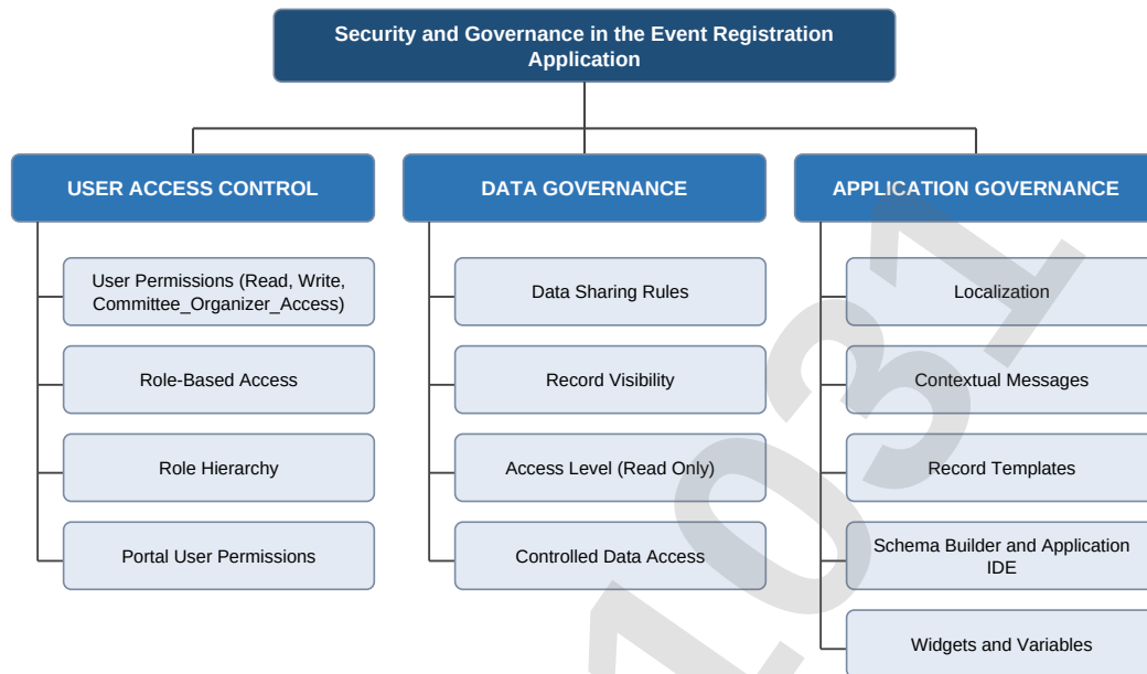
Figure 6: Classification of Security and Governance Controls (Conceptual Diagram)
