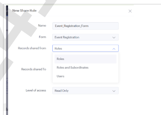
Figure 5: New Share Rule panel – options for Records shared from
